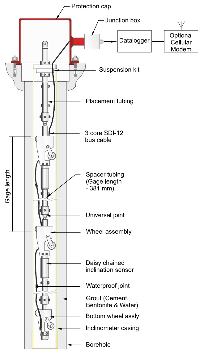
EAN-52M In-place inclinometer system with SDI-12 bus interface to SDI-12 compatible datalogger
