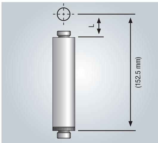
Ref.-No. 484 715 Connection Leica pin for Leica GPH1A Omni #3425 L = 125 mm
